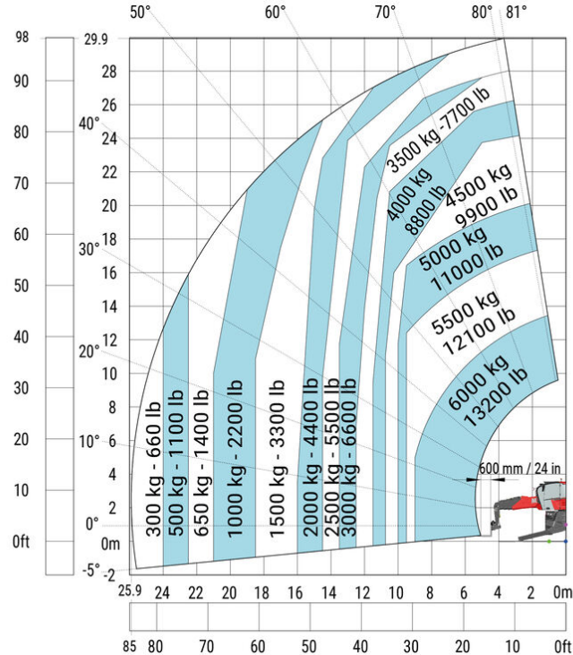
Machine on lowered stabilizers with forks
