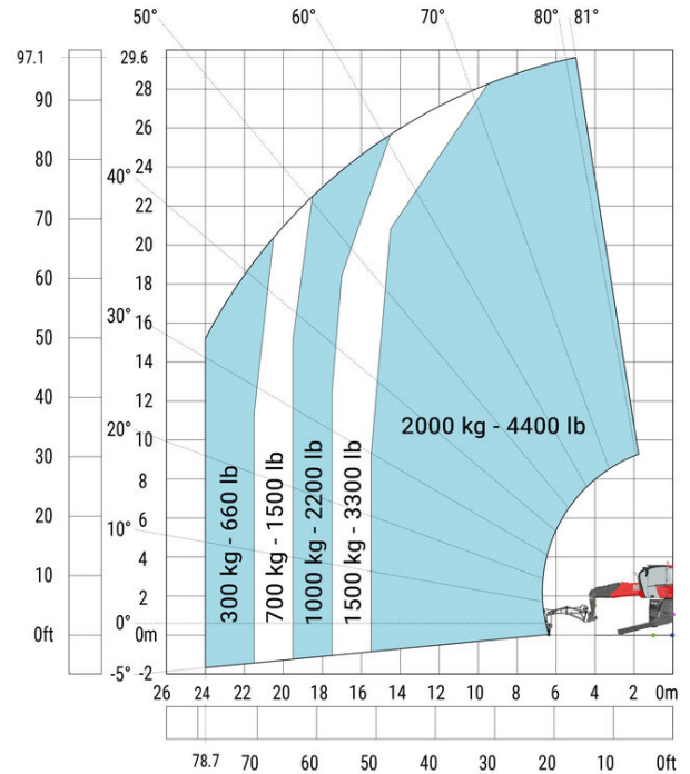
Machine on lowered stabilizers with 4,400 lb jib
