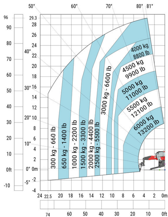
Machine on lowered stabilizers with winch 13,200 lb
