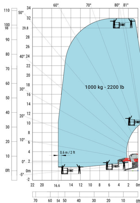
Machine on lowered stabilizers with 2,200 lb platform
