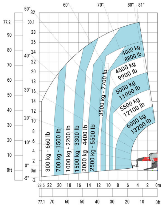
Machine on lowered stabilizers with hook 13,200 lb
